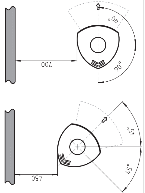
Min. distance to combustible wall with revolvable pedestal
