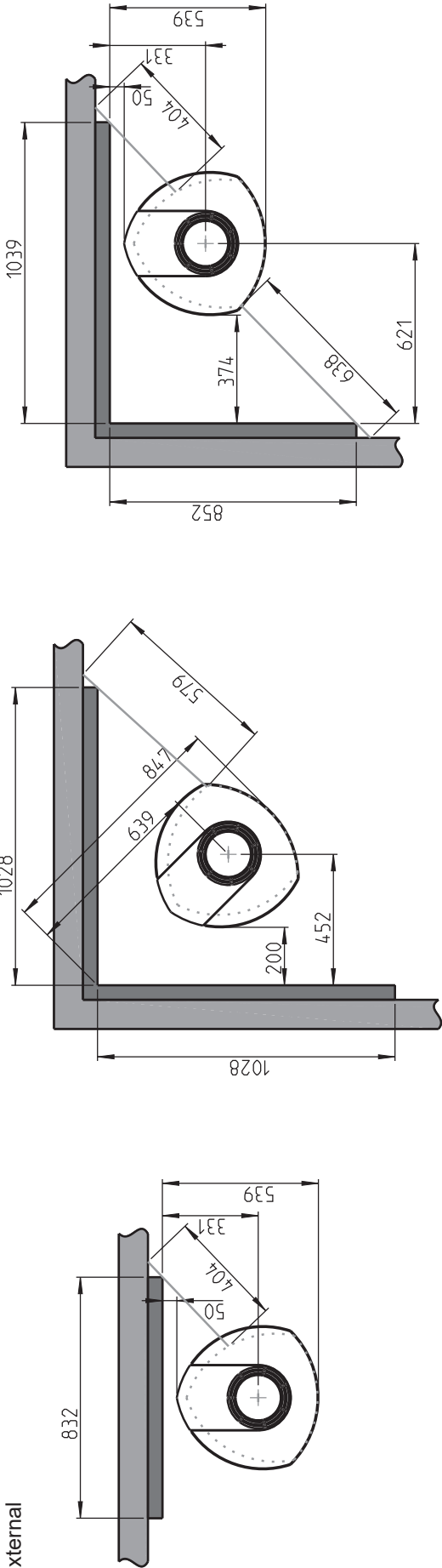
Jøtul F 377 Advance - min. distance to firewall
